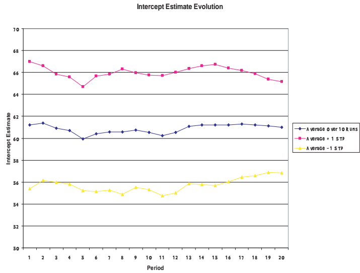
Figure 1: The estimate \hat{\beta}_t^0 .
