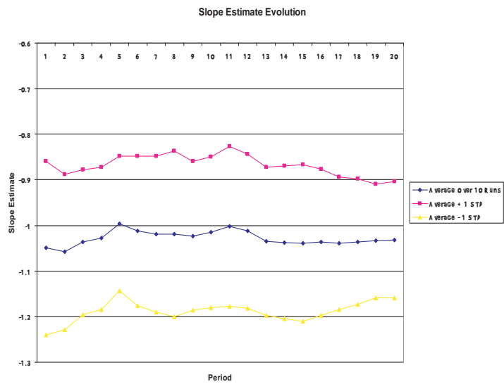
Figure 2: The estimate \hat{\beta}_t^1 .
